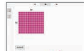
Multiplication Models
